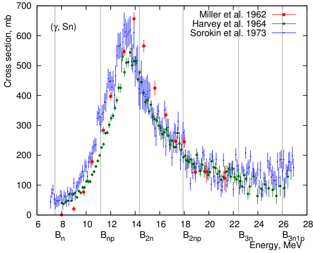
Figure 2. Photoneutron yield reaction cross sections \sigma(\gamma, Sn) measured by Miller et al. [8], Harvey et al. [9], and Sorokin et al. [10].
