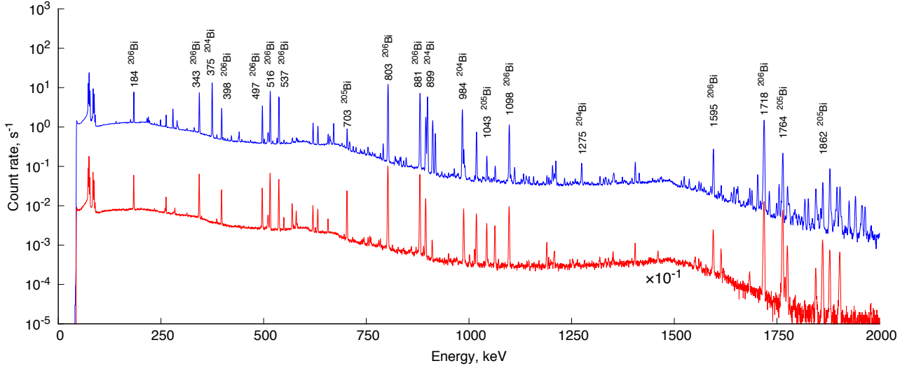
Figure 1. Two sample spectra of induced gamma-ray activity of the irradiated bismuth target summed over 10 hr immediately after the irradiation (upper curve) and 1 week after the irradiation (lower curve, multiplied by 10^{-1} ).
