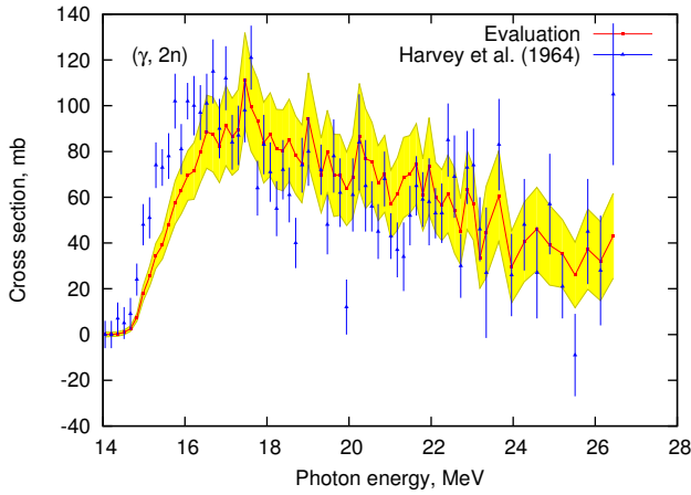
Figure 5. Evaluated partial photoneutron reaction cross sections \sigma(\gamma, 2n) compared to the experimental cross sections from [9]. The uncertainty of the evaluated cross section is denoted with yellow-filled band.
