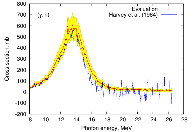
Figure 4. Evaluated partial photoneutron reaction cross sections \sigma(\gamma, 1n) compared to the experimental cross sections from [9]. The uncertainty of the evaluated cross section is denoted with yellow-filled band.
