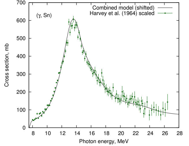
Figure 3. Photoneutron yield reaction cross section \sigma(\gamma, Sn) from [9] scaled by 1.12 and matching of the theoretical cross section to it when shifted by 0.15 MeV.
