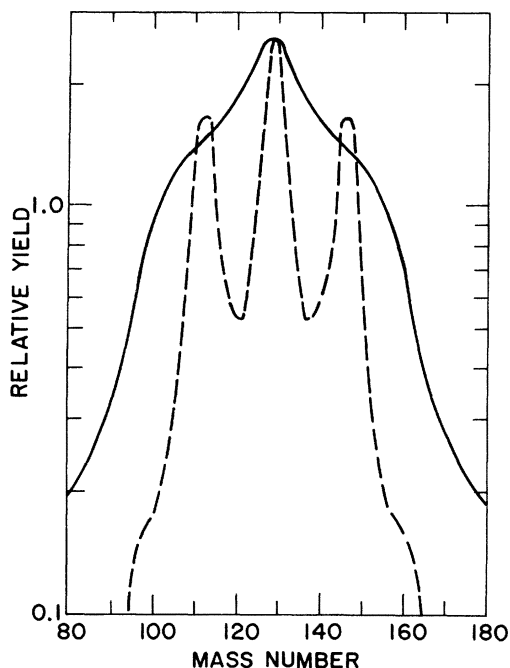
FIG. 15. Comparison of the calculated mass distribution for ^{258}\text{Fm} (dashed line) with the experimental data for ^{257}\text{Fm}(n_{th}, f) (Ref. 35) (solid line).
