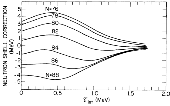
FIG. 3. The neutron-shell corrections at a fixed deformation ( \beta = 0.65 ) calculated as a function of the intrinsic temperature, \tau_{\text{int}} . These shell corrections correspond to those in the vicinity of point H of Fig. 1.
