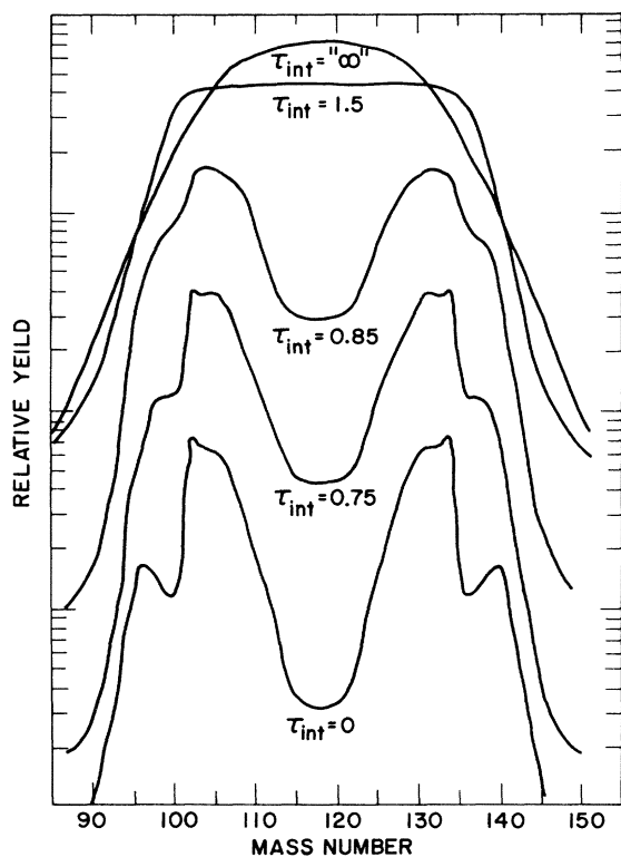
FIG. 11. The mass distribution for ^{238}\text{U} calculated at several different temperatures \tau_{\text{int}} . The calculation at \tau_{\text{int}} = \infty has the shell and pairing corrections set to zero.
