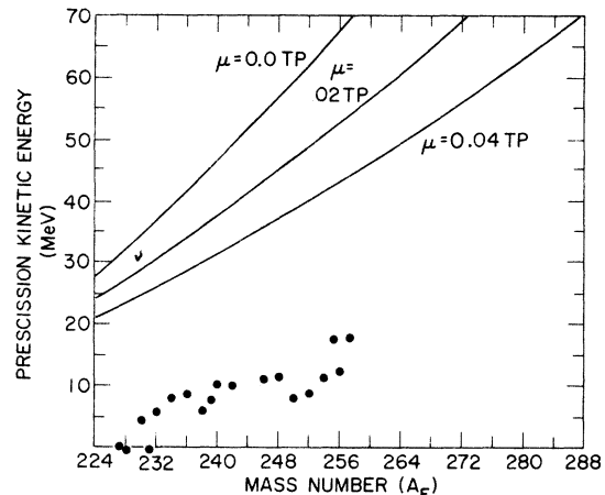
FIG. 30. Prescission kinetic energy as a function of A_F . The points represent estimates of the prescission kinetic energy based on the scission shapes derived from our model. The solid lines are the calculated prescission kinetic energies for three different values of the viscosity coefficient as obtained in the dynamic calculation of Davies et al. (Ref. 40).
