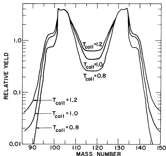
FIG. 17. The calculated mass distribution of ^{236}\text{U} for different values of the parameter, T_{\text{coll}} , holding the value of the other parameters fixed (see text). The relative mass distributions have been normalized at mass 134.
