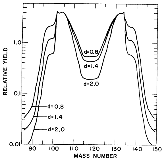
FIG. 16. The calculated mass distribution of ^{236}\text{U} for different values of d (the distance between the tips of the two spheroids) holding the value of the other parameters fixed (see text). The relative mass distributions have been normalized at mass 134.
