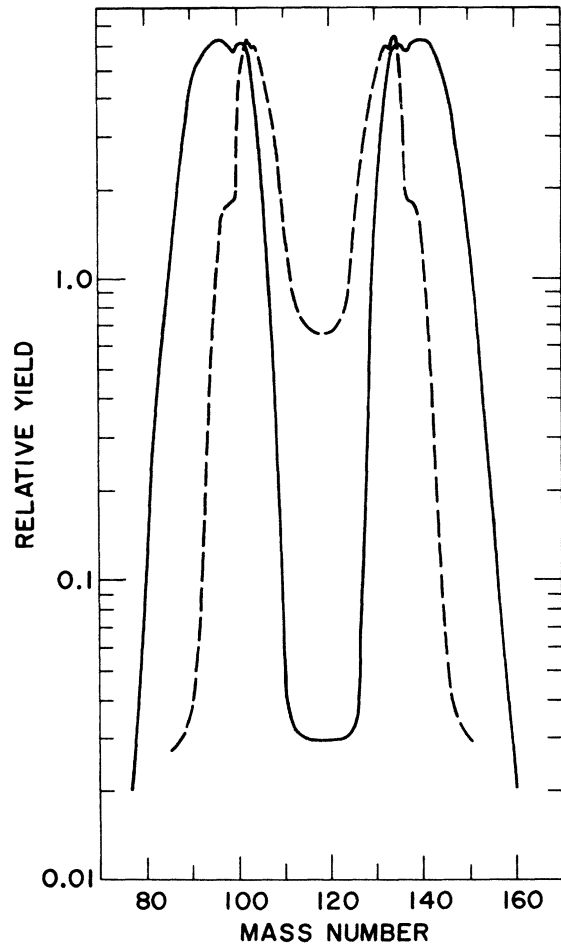
FIG. 13. Comparison of the calculated mass distribution for ^{236}\text{U} (dashed line) with the experimental data for ^{235}\text{U}(n_{\text{th}}, f) (Ref. 37) (solid line).
