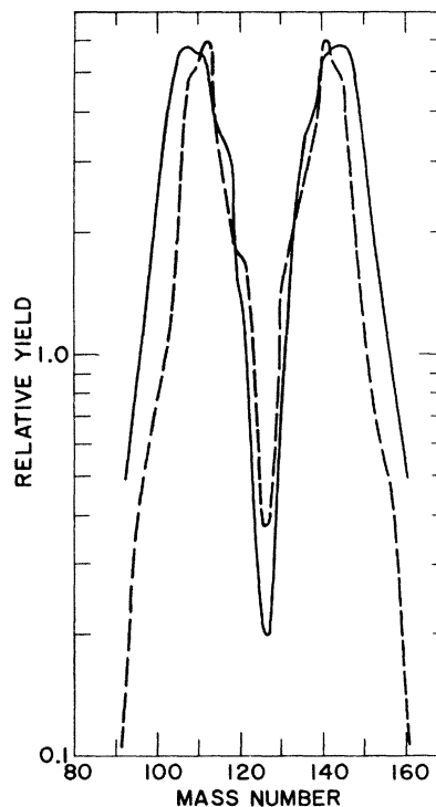
FIG. 12. Comparison of the calculated mass distribution for ^{252}\text{Cf} (dashed line) with the experimental data for ^{252}\text{Cf(sf)} (Ref. 33) (solid line).
