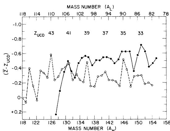
FIG. 32. The quantity (\bar{Z} - Z_{UCD}) for different mass splits in the fissioning system ^{236}\text{U} as calculated from our model (dashed line) compared with the experimental results of Clerc et al. (Ref. 65) for ^{235}\text{U}(n_{th}, f) (solid line). The locations of the odd values of Z_{UCD} are shown in the figure.
