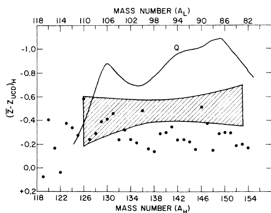
FIG. 31. A plot of (\bar{Z} - Z_{UCD}) as a function of mass split for the system ^{236}\text{U} . The points are calculated from our model. The elongated box encloses the data of Reisdorf et al. (Ref. 37), obtained from K x rays. The solid line ( Q ) gives the nuclear charge division associated with the maximum energy release for odd-mass fragments (see text).
